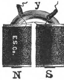
FIG. 42.—HORSESHOE ELECTROMAGNET.
