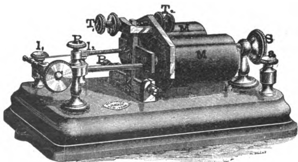
FIG. 55.—TELEGRAPHIC RELAY.
