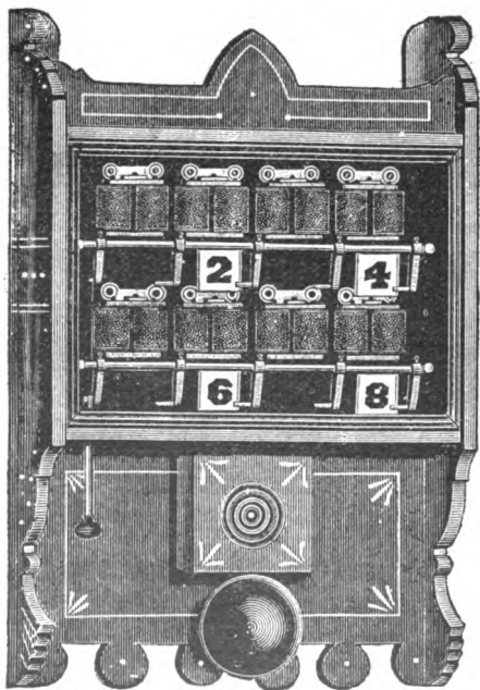
FIG. 58.—ELECTROMAGNETIC ANNUNCIATOR.
