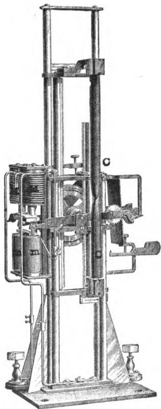
FIG. 60.—ARC-LAMP MECHANISM.
