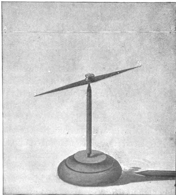
FIG. 29.—DEFLECTION OF MAGNETIC NEEDLE WHEN SUPPORTED BENEATH A WIRE CONVEYING AN ELECTRIC CURRENT.
