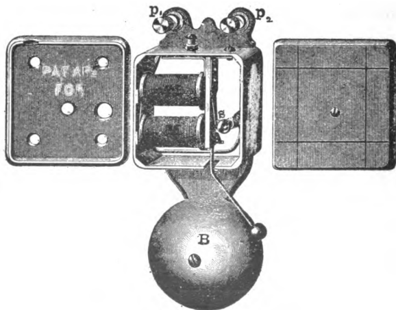
FIG. 57.—ELECTROMAGNETIC BELL.
