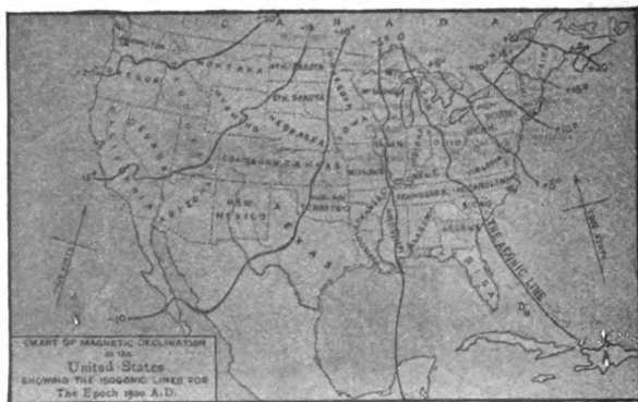
FIG. 81.—ISOGONIC CHART OF THE UNITED STATES FOR THE YEAR 1900.
