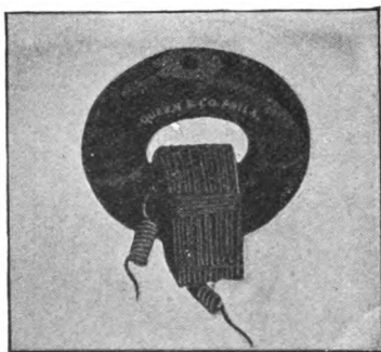
FIG. 52.—FERRIC MAGNETIC CIRCUIT.
