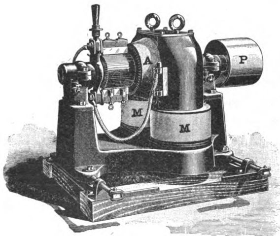
FIG. 67.—ELECTROMAGNETIC MOTOR.
