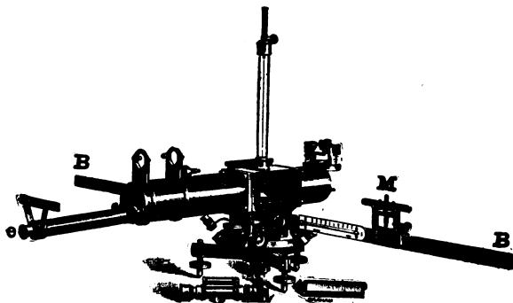
FIG. 85.—MAGNETOMETER.
