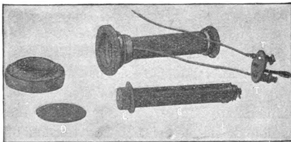
FIG. 56.—PARTS OF AN ORDINARY BELL TELEPHONE.
