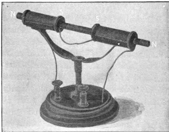
FIG. 44.--ANOMALOUS ELECTROMAGNET.
