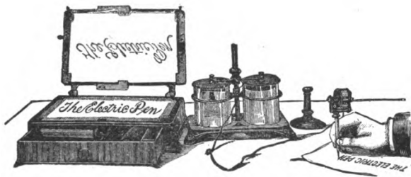
FIG. 59.—EDISON'S ELECTRIC PEN AND DUPLICATING PRESS.
