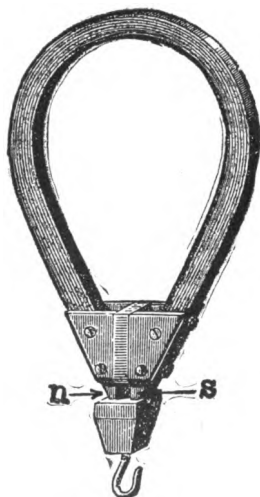
FIG. 49.—COMPOUND PERMANENT MAGNET WITH CONSTANT POLE SURFACES.
