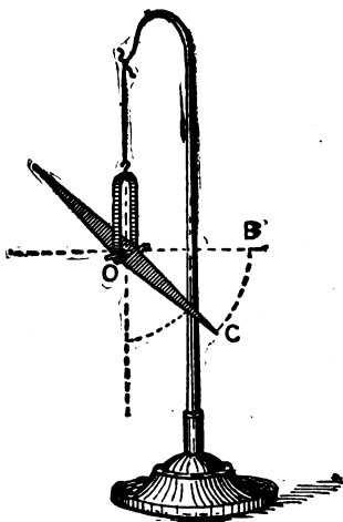
FIG. 82.—DIPPING NEEDLE.
