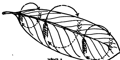
FIG 1 ROTATION IN 3 SPACE ABOUT A LINE
