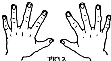
FIG 2 ROTATION IN 4 SPACE ABOUT A PLANE
